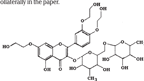
Fig. 2. Troxerutin (3',4',7-Tris [O-(2-hydroxyethyl)]rutin) structure
